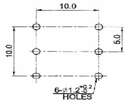
P.W.B MOUNTING DETAIL
